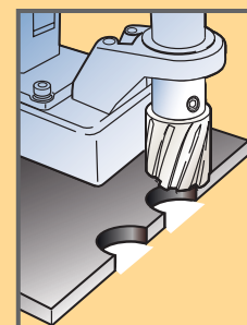
Edge-hole cutting
