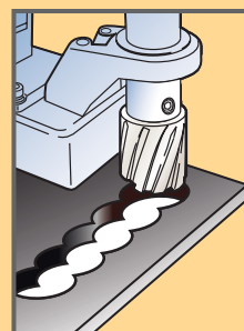
Overlapped cutting
